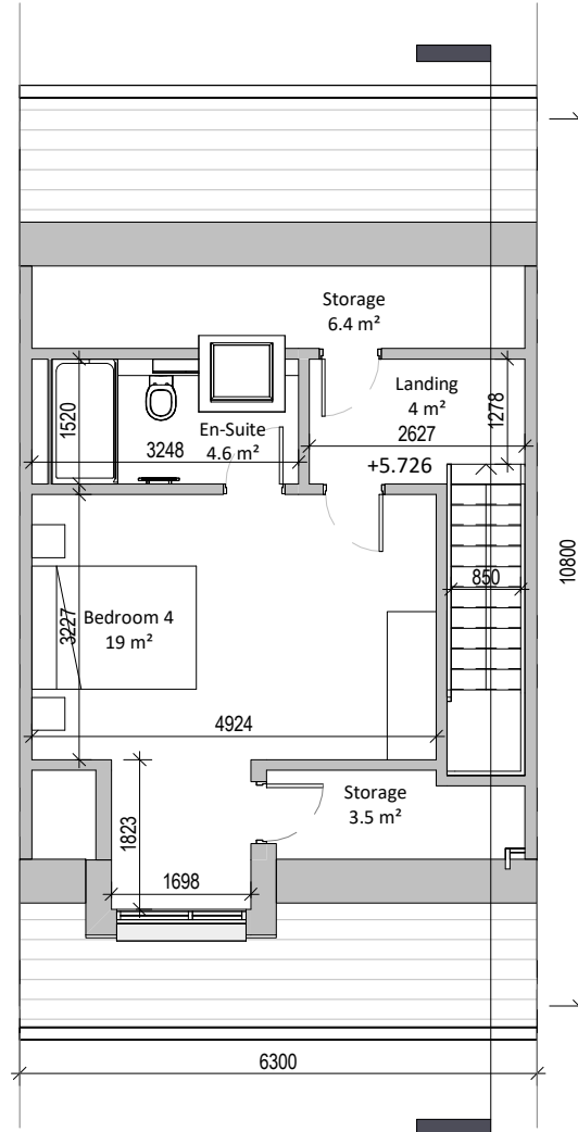
3 Second Floor Plan 1 : 100
