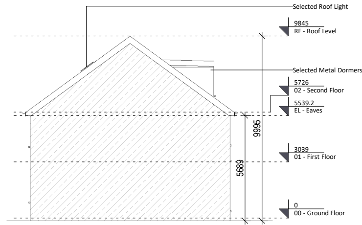
6 Left Elevation / Party Wall Section 1 : 200
