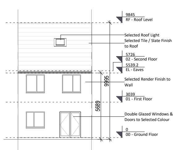
5 Rear Elevation 1 : 200
