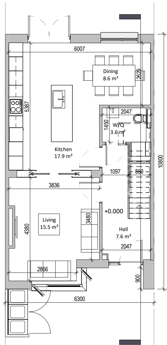
1 Ground Floor Plan 1 : 100
