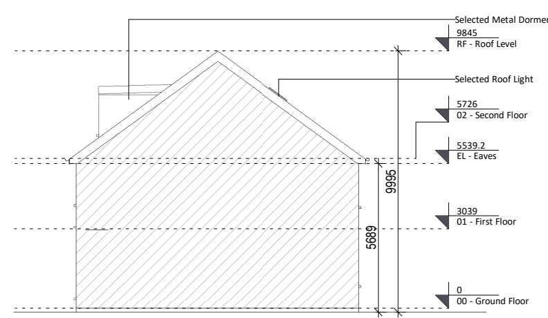
7 Right Elevation / Party Wall Section 1 : 200
